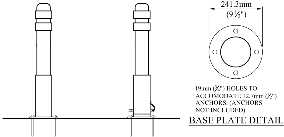
SURFACE MOUNT PERMANENT (BDC3PS)
