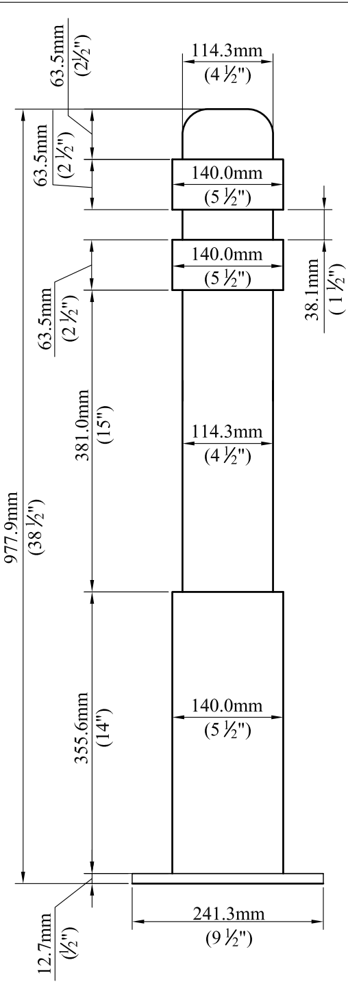
SURFACE MOUNT PERMANENT (BDC3PS)
