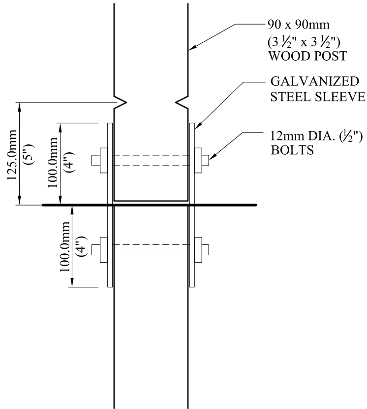
BREAKAWAY DETAIL (SIDE VIEW)
