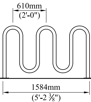
ELEVATION - 3 MOUND
