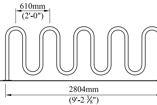
ELEVATION - 5 MOUND
