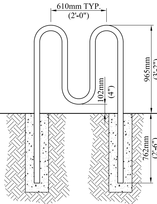
ELEVATION - 2 MOUND
