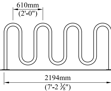
ELEVATION - 4 MOUND
