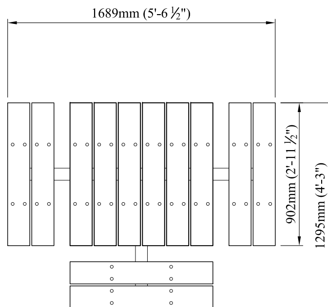
PLAN VIEW WHEELCHAIR ACCESSIBLE
