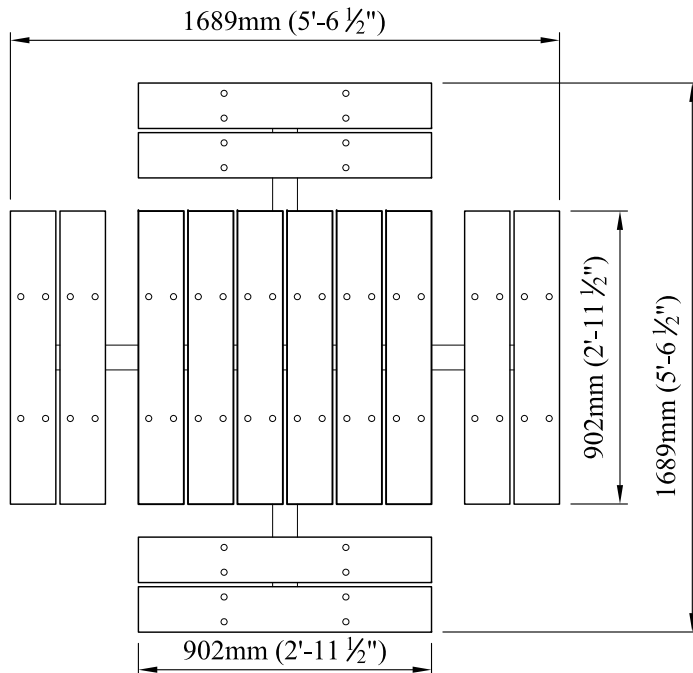
PLAN VIEW
