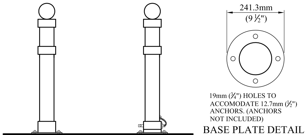
SURFACE MOUNT PERMANENT (BDB2PS)
