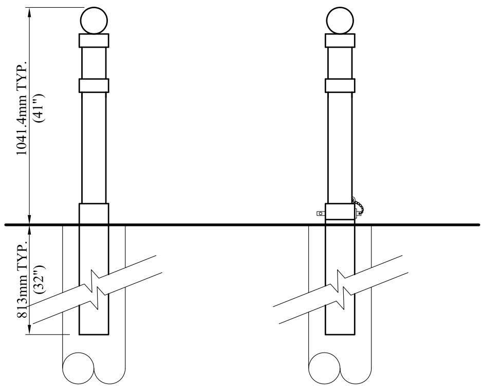
IN GROUND PERMANENT (BDB2PG)
