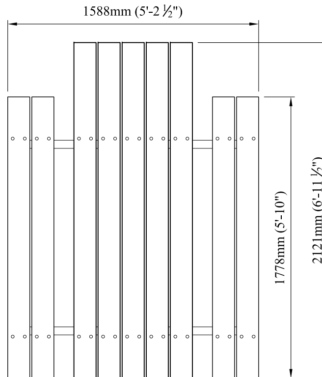
PLAN VIEW WHEELCHAIR ACCESSIBLE
